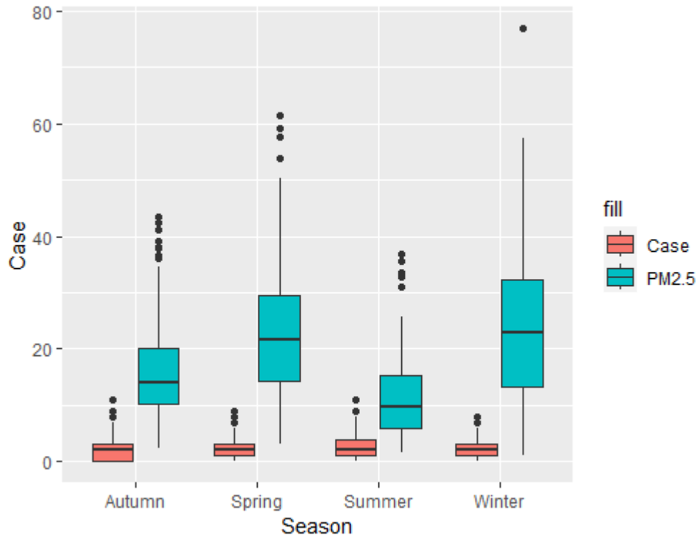
Figure S2. The season variation of PM 2.5 concentration and the frequency of admissions for asthma in Xiamen, China.
