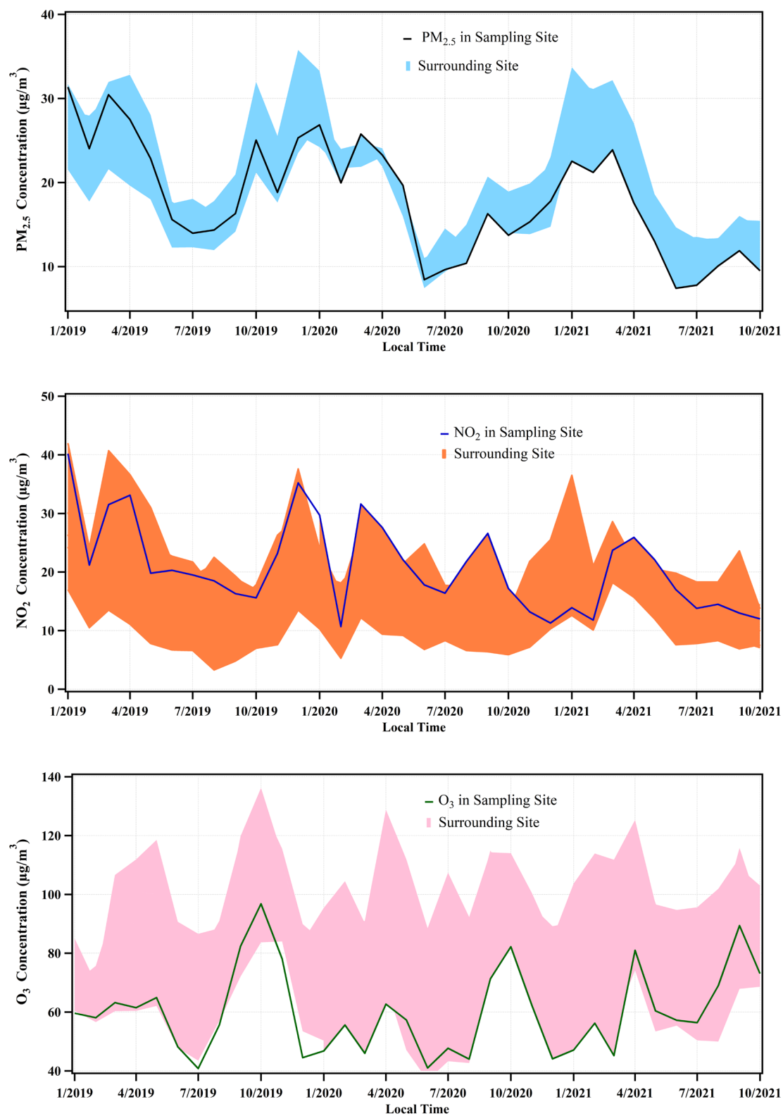
Figure S1. Time series of PM 2.5 and gaseous pollutants concentrations (monthly mean values) in sampling site and surrounding observation site during the study period.
