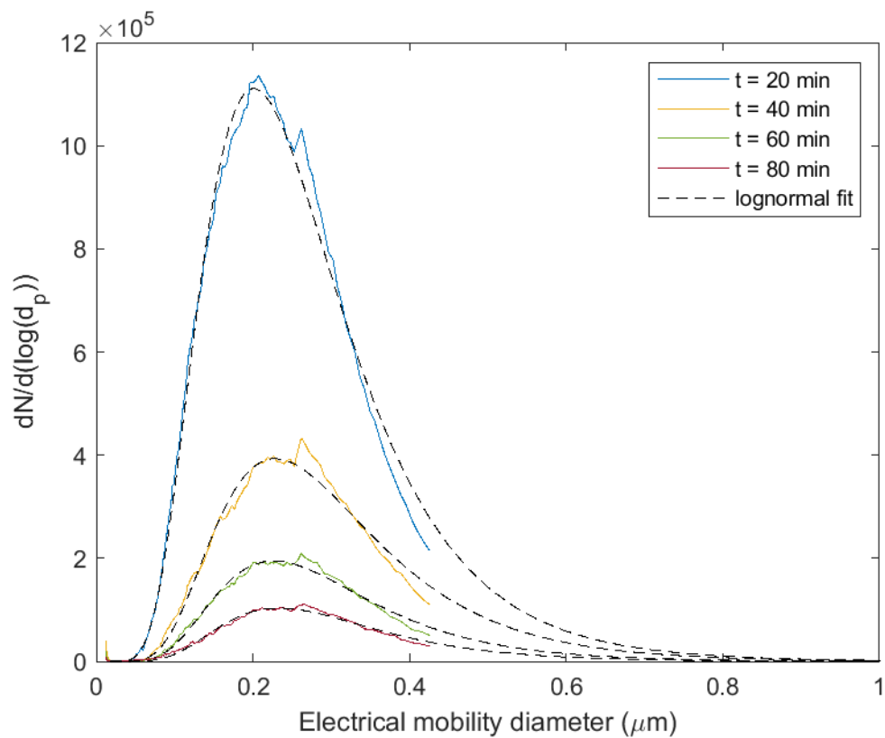
Fig. S2. Particle size distributions measured by Scanning Mobility Particle Sizer (solid lines) and fitted lognormal distributions (dashed lines) during chamber experiment.
