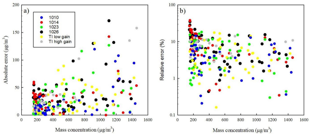
Fig. S1. Absolute (a) and relative (b) error of each sensor as a function of reference mass concentration.
