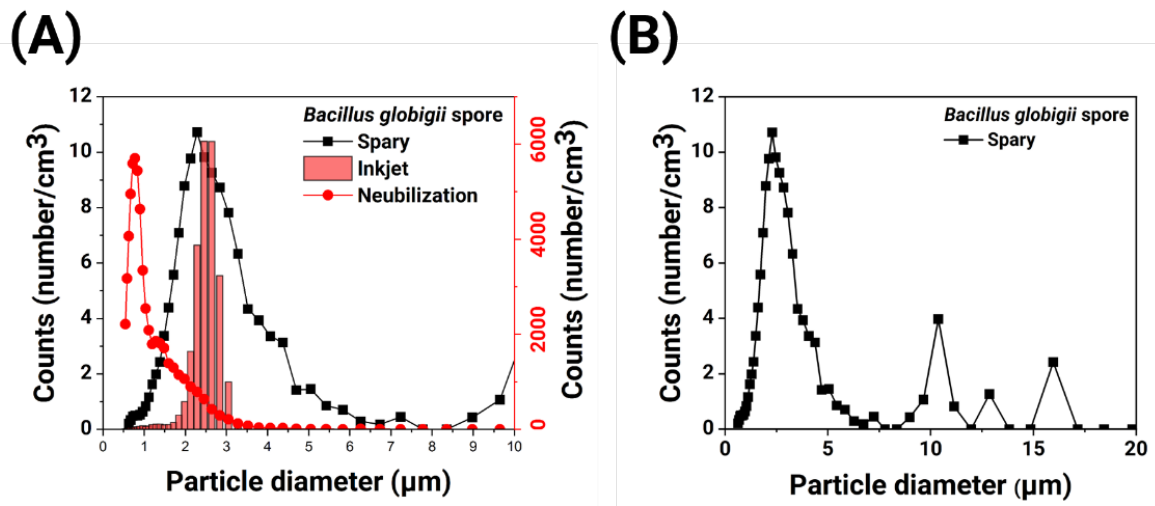
Fig. S1. Size distribution of BG spore aerosols generated by mechanical spray, inkjet and nebulization methods.
