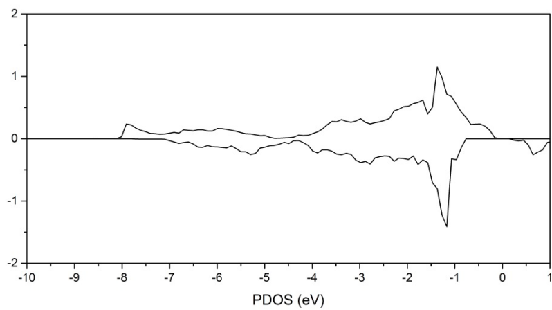
Fig. S1. PDOS of O 3 C on clean CuO(111) surface.
