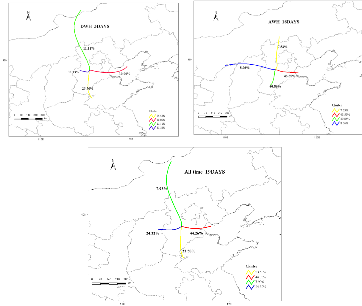
Fig. S2. Clustering analysis of backward trajectories for DWH, AWH, and whole sampling period.
