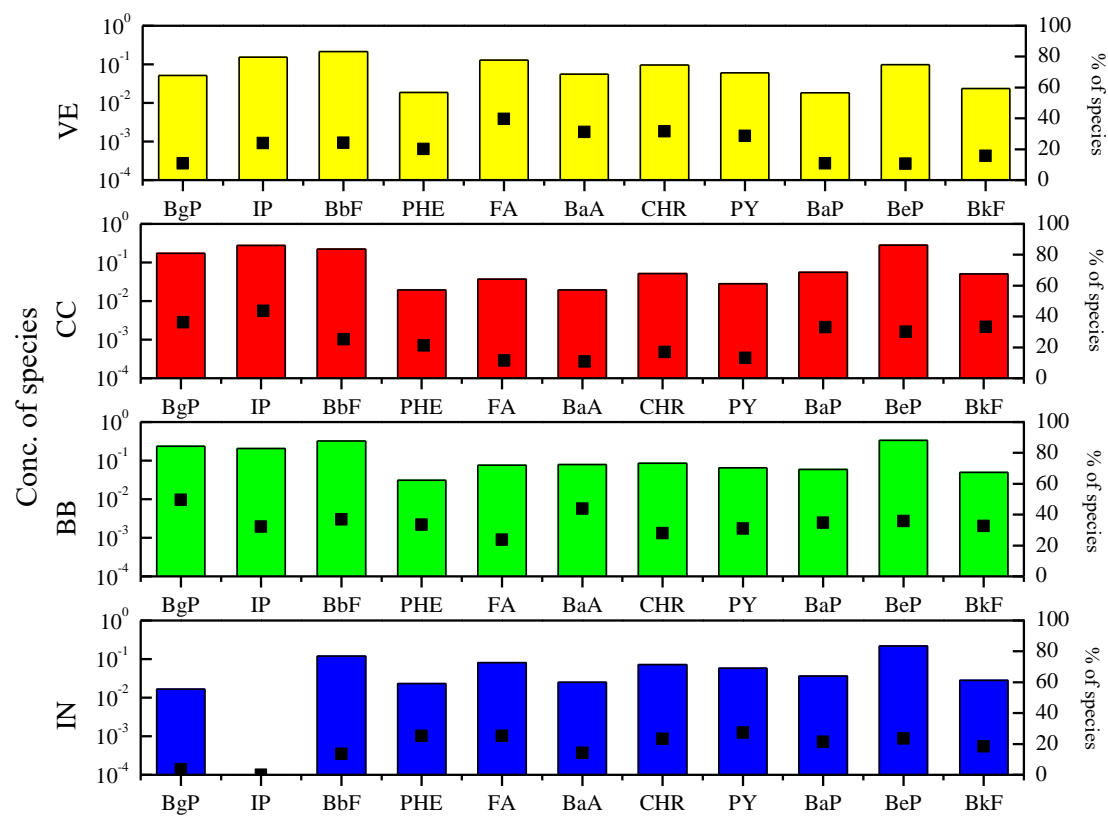
Fig. S1. Source profiles of four PAH sources identified by PMF model for whole sampling period.
