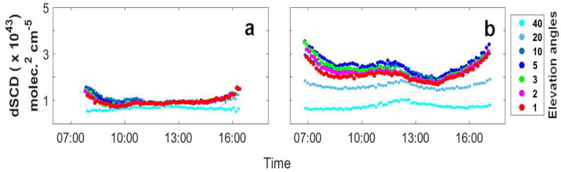
Figure S1: Diurnal variation of O_4 dSCDs from (a) 7 th January 2018 and (b) 20 th April 2018. The diurnal variation of O_4 on 7 th January 2018 shows two daily maxima (hence ‘U’ shape) whereas, on 20 th April 2018 shows three daily maxima (hence ‘W’ shape).
