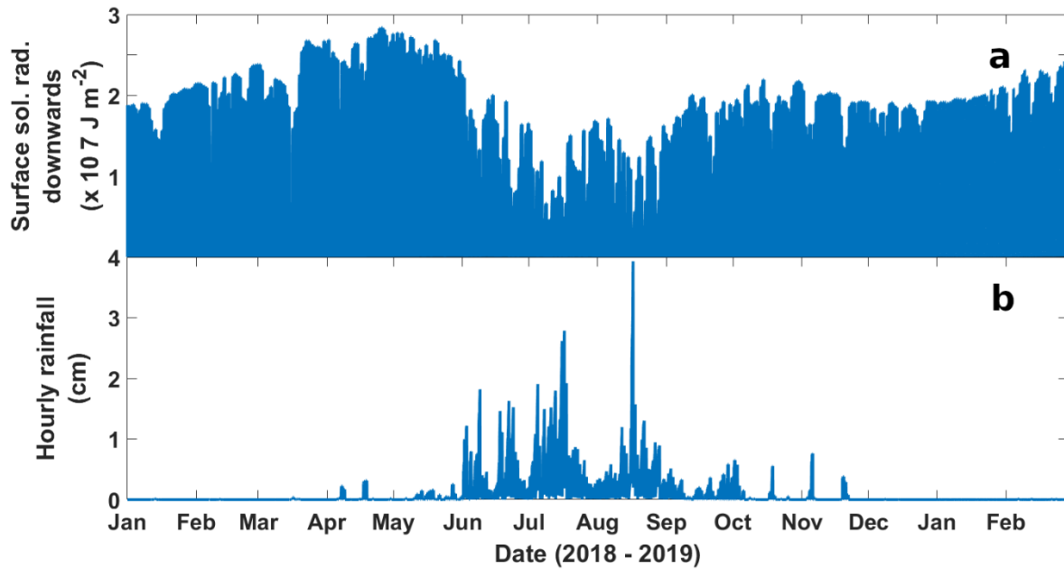
Figure S2: Time series of (a) surface solar radiation downwards and (b) total precipitation averaged over 0.3^\circ \times 0.3^\circ box around the Pune observation site. The data used here is ERA5 reanalysis product at 0.1^\circ \times 0.1^\circ resolution. We can see that solar radiation is lower and rainfall during JJAS compared to rest of the period.
