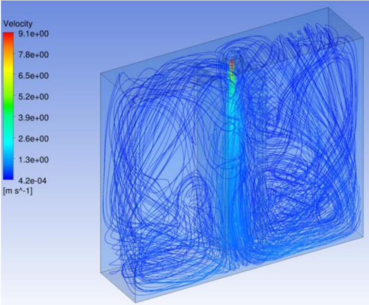
Figure S2. CFD simulations results of the velocity streamlines
