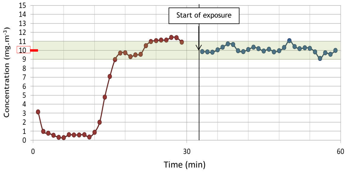
Figure S3. APS aerosol mass concentration monitoring
