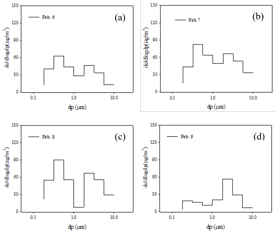
Figure S-1. The size distribution of marine particulate matter on February 6-9 at the Nankan Island.
