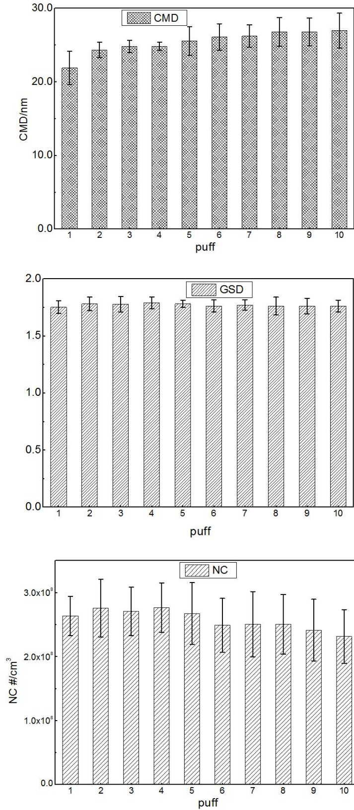
Fig. S2. The puff-by-puff CMD, GSD and NC of aerosol from the 4#E-cigarette.
