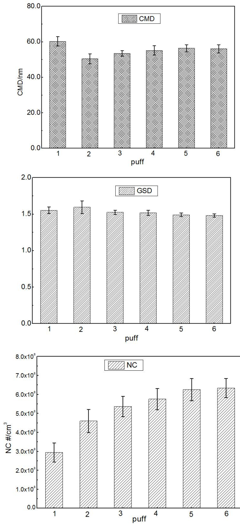
Fig. S3. The puff-by-puff CMD, GSD and NC of aerosol from the 7#HNB cigarette.
