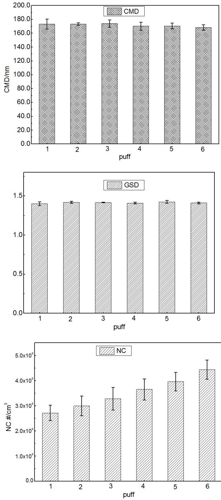
Fig. S1. The puff-by-puff CMD, GSD and NC of smoke particles from the 3R4F reference cigarette
