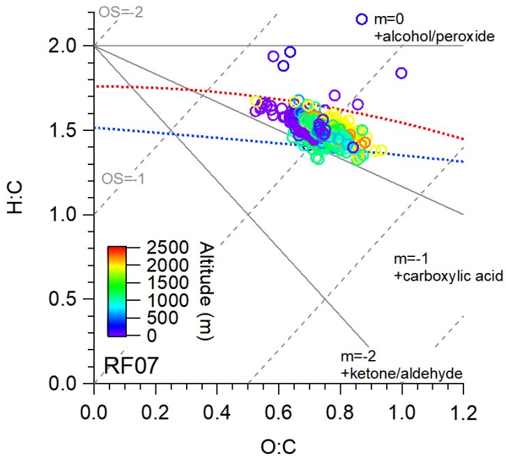
Fig. S2. Van Krevelen diagram for data measured during RF07.
