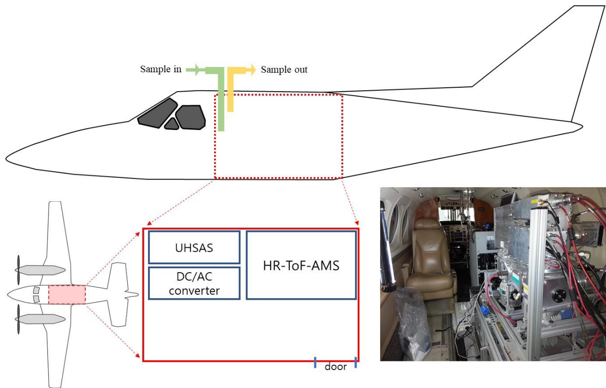
Fig. S1. Schematic of the Hanseo KingAir-C90GT aircraft.
