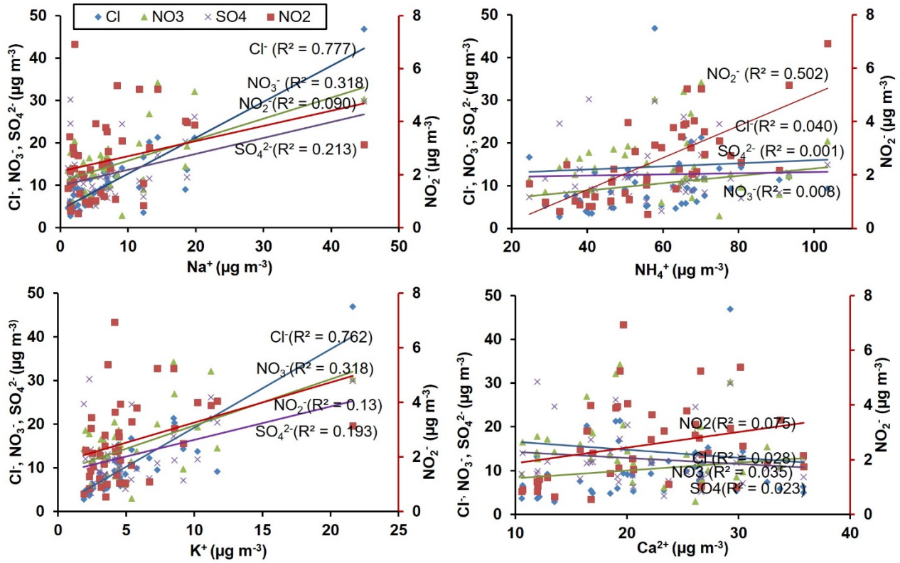
Fig. S1. Regression analysis of major anions with each of cations at the urban site.
