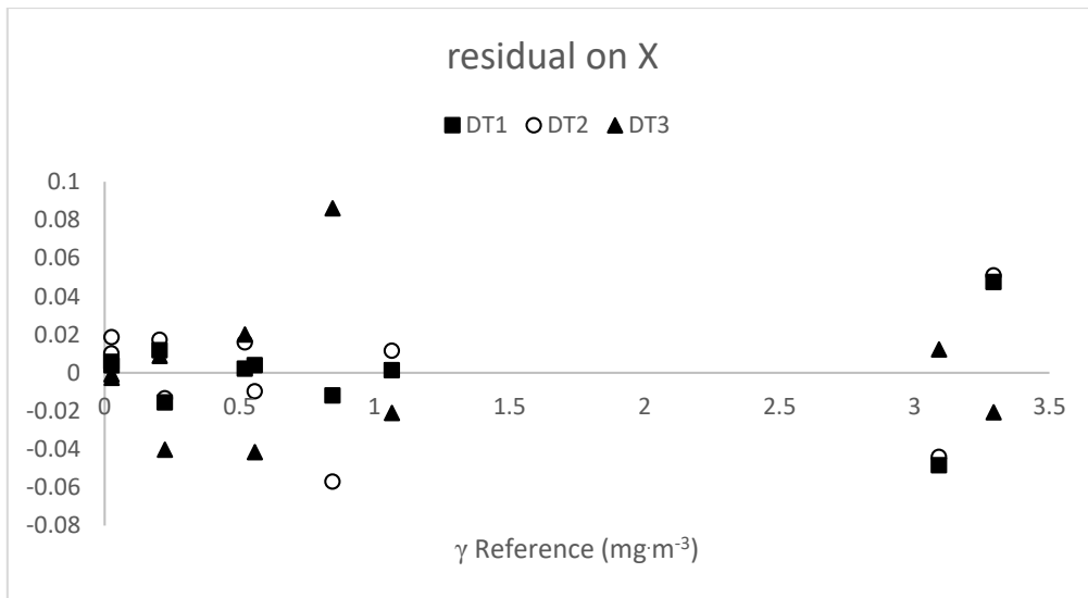
Figure S1. Residual analysis plot for the linear regression model of the responses for three DustTrak DRX units (DT1, DT2, DT3) when measuring Emery oil aerosol mass concentration.
