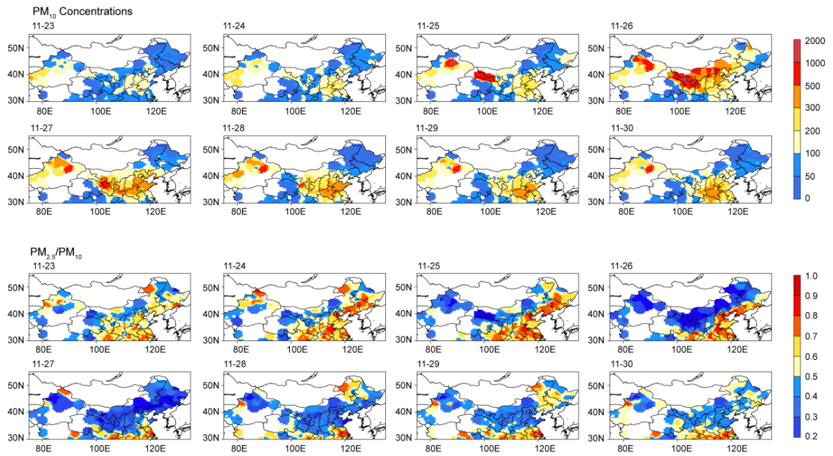
Fig. S1 Daily interpolated distributions of the observed PM_{10} concentration and PM_{2.5}/PM_{10} ratio near the surface on November 23 to 30, 2018.
