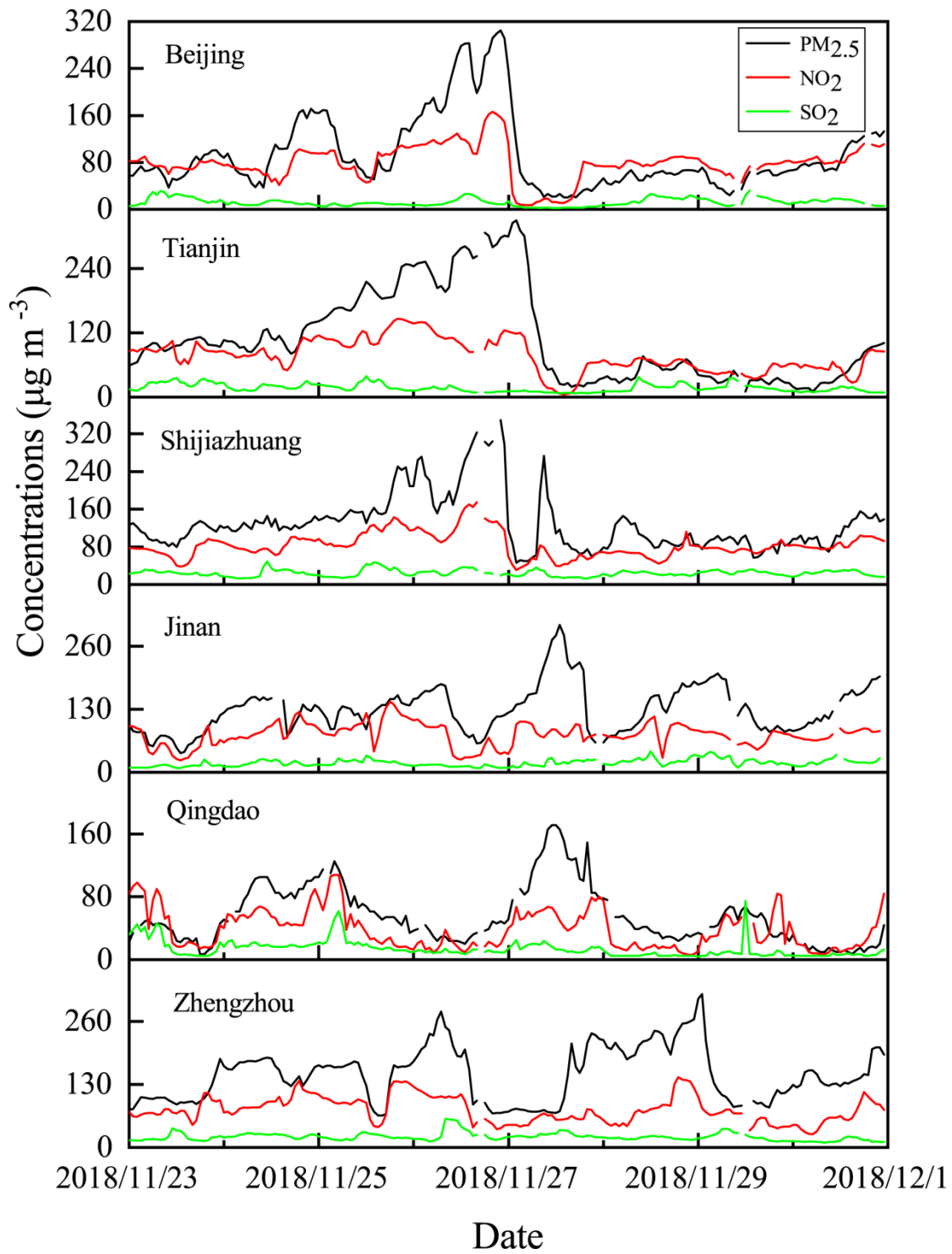
Fig.S2. Hourly concentrations ( \mu\text{g m}^{-3} ) of PM 2.5 (black line), NO 2 (red line), and SO 2 (green line) in Beijing, Tianjin, Shijiazhuang, Qingdao, Zhengzhou, and Jinan from November 23 to 30, 2018.
