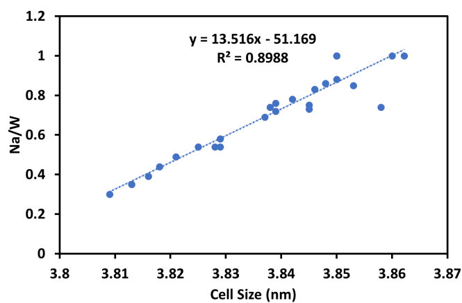
Figure S1. Summary of lattice size of cubic sodium tungsten bronze in the ICDD database
