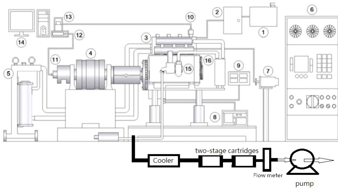
Diagrammatic representation of diesel engine.
