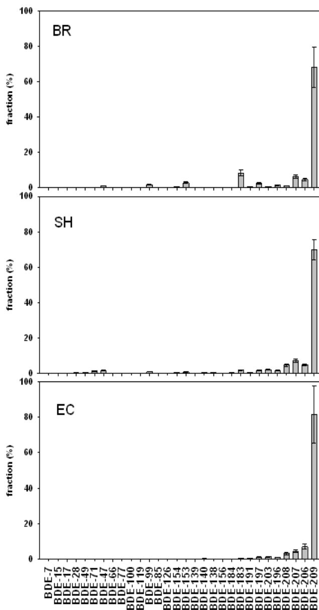
Fig. 7. PBDE congener profiles of the ashes in the MSWI-B operating units (a).
