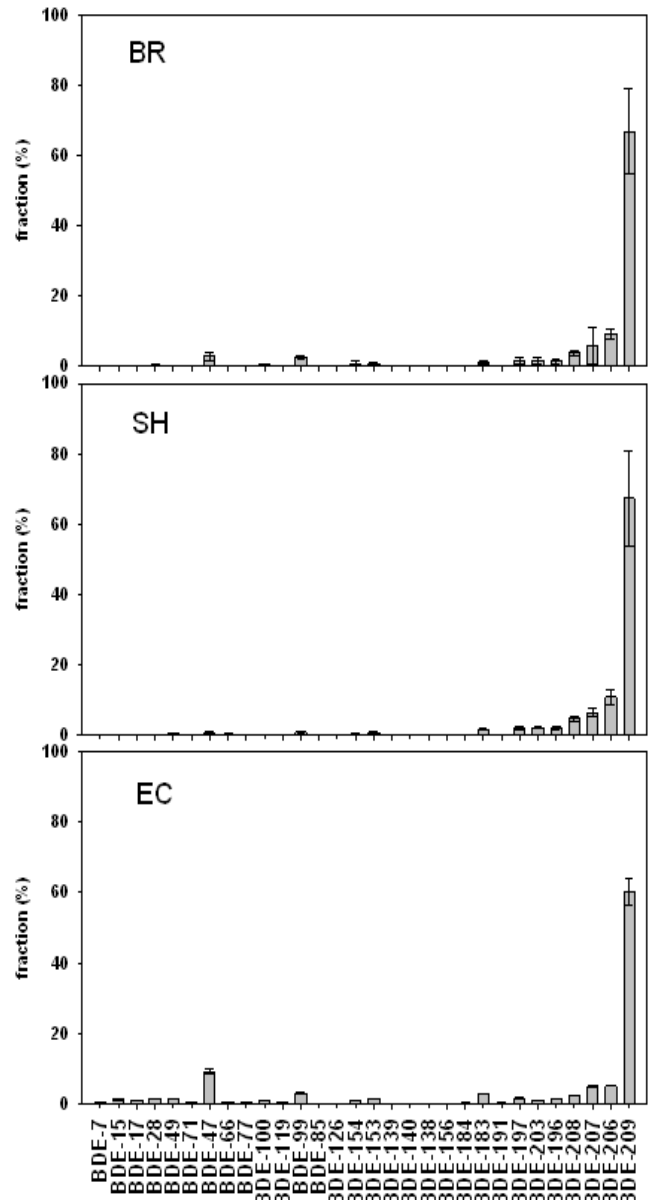
Fig. 5. PBDE congener profiles of the ashes in the MSWI-A operating units (a).
