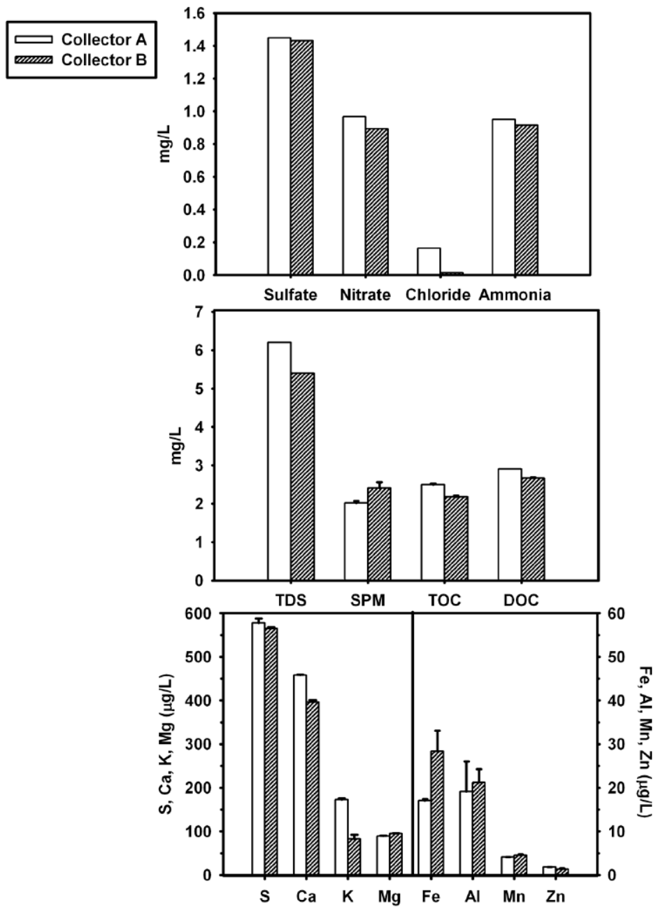
Fig. S1. Characterization of the rain water collected at Devil's Lake State Park July 9, 2004 for the following constituents: sulfate, nitrate, ammonium, chloride, total dissolved solids (TDS), suspended particulate matter (SPM), total organic carbon (TOC) and dissolved organic carbon (DOC), and soil derived cations.
