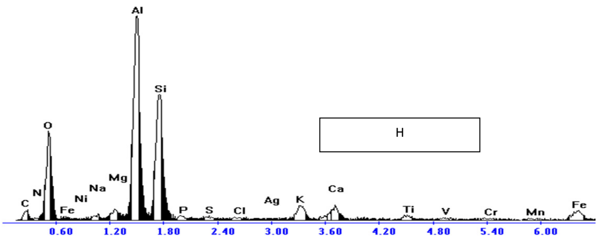
Supp 4. Examples of EDS spectra: residual fraction of NIST 1649 a (3 h of US supply).
