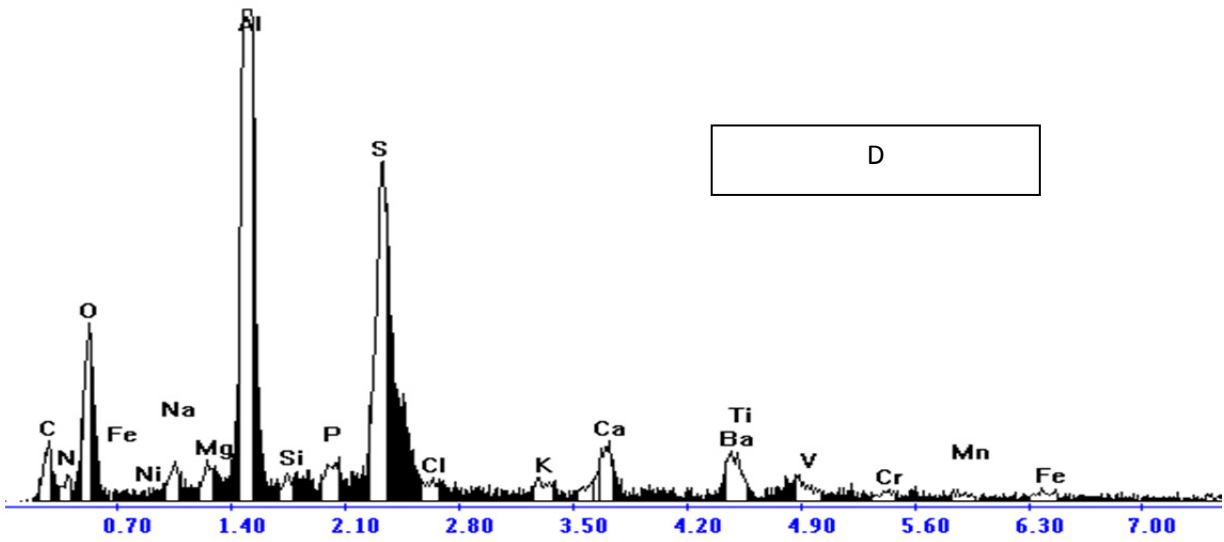
Supp 2. Examples of EDS spectra: suspended fraction of NIST 1649 a (3 h of US supply).
