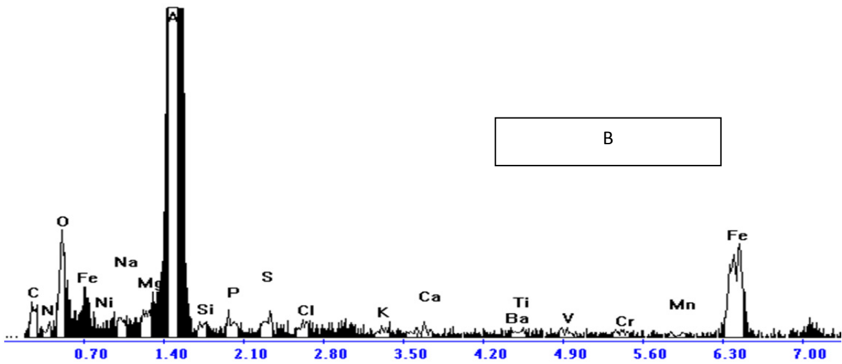
Supp 1. Examples of EDS spectra: suspended fraction of NIST 1649a (3 h of US supply).
