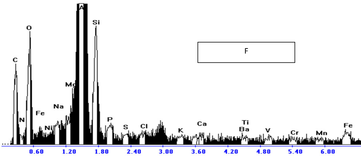
Supp 3. Examples of EDS spectra: residual fraction of NIST 1649 a (3 h of US supply).
