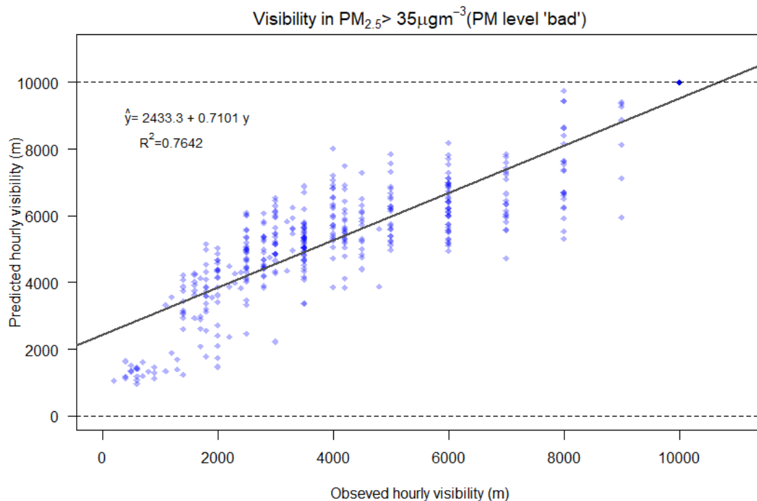
Fig. 8. Observed and predicted hourly visibility for PM 2.5 > 35 µg m -3 at IIA using censored regression model (Model 8 of Table 2) from 1 January till 25 May 2018.
