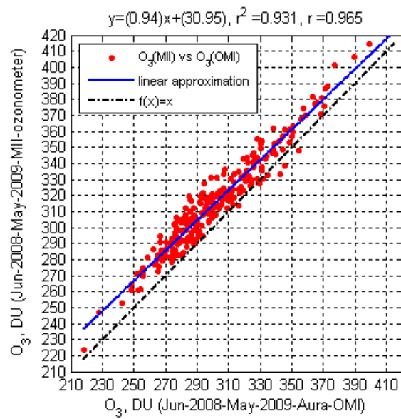
Figure S1. Relation of total ozone according to Microtops II Ozonometer and AURA OMI data, July 2008 – May 2009
