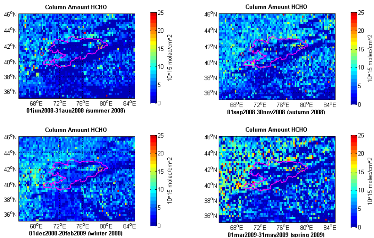
Figure S3. Seasonal maps of column amount HCHO distribution (Aura OMI satellite).
