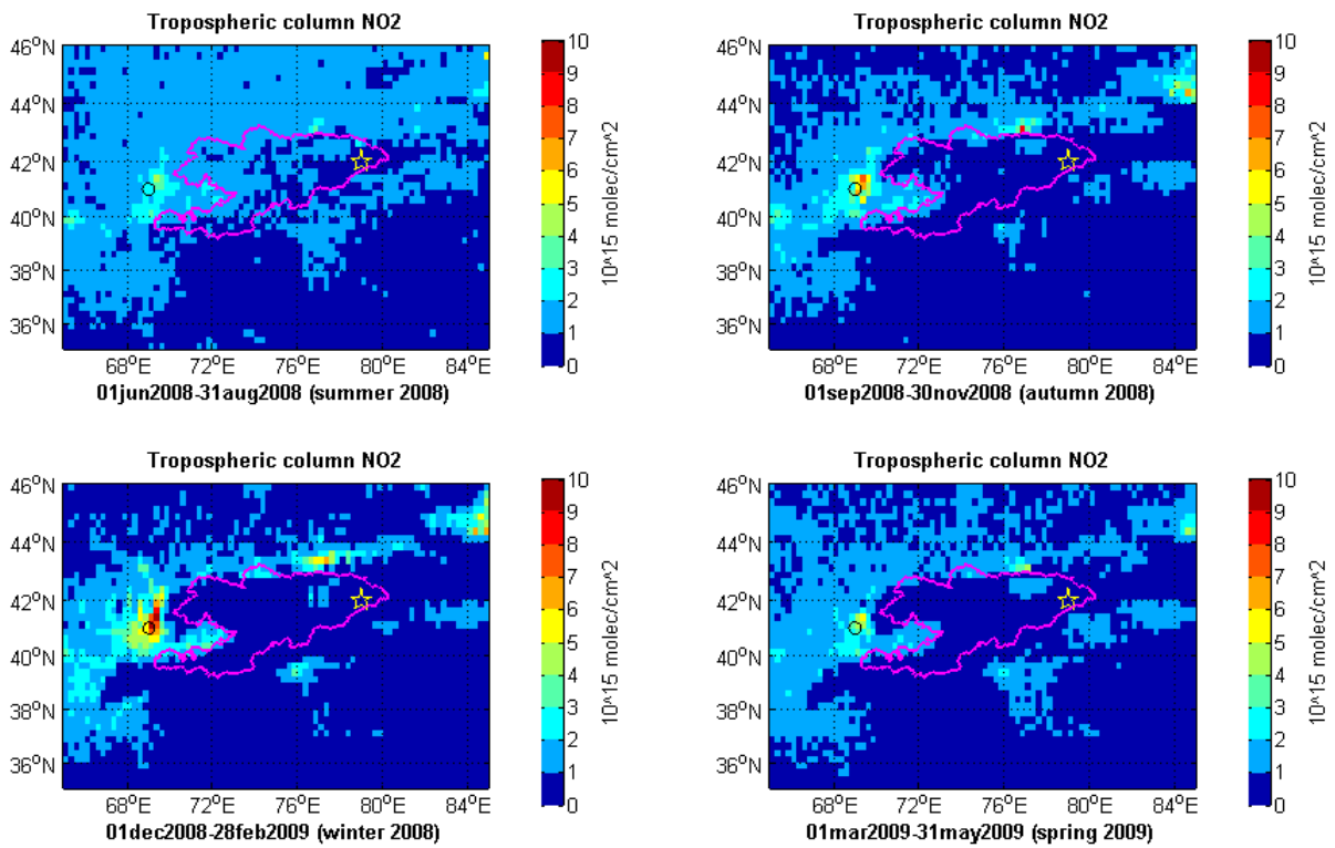
Figure S2. Seasonal maps of tropospheric column NO 2 distribution (Aura OMI satellite).
