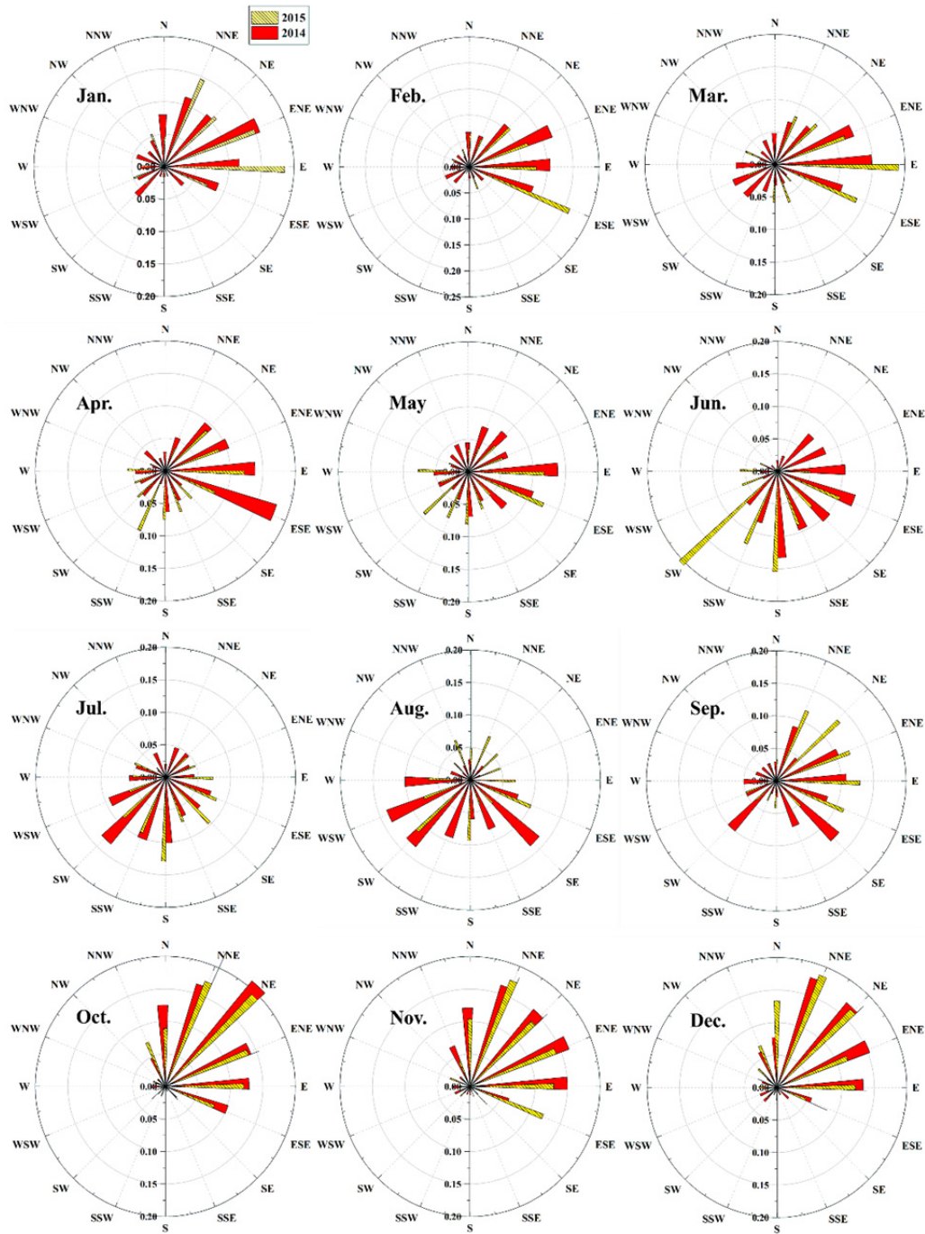
Fig. S2. The monthly wind rose diagram for Xiamen, China in 2014-2015. The data was recorded from https://rp5.ru/ .
