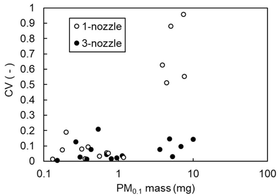
532 Fig. 12. Correlation between particle mass and coefficient of variation of carbon mass collected 533 on different locations on the backup filter.
