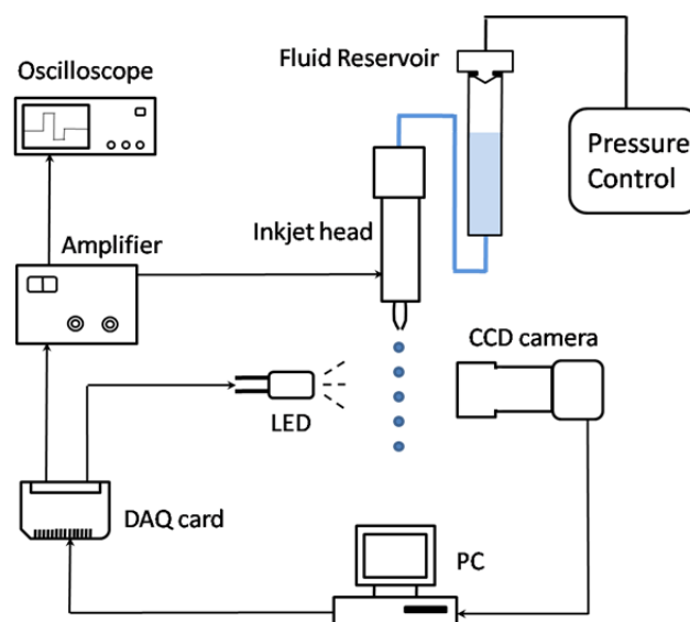
Fig. 1. Schematic diagram of the inkjet system.
