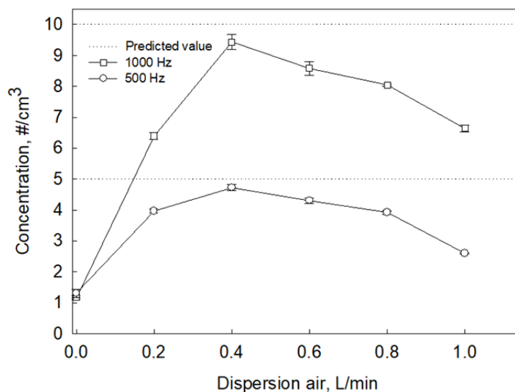
Fig. 4. Effect of dispersion air on the aerosol concentration.
