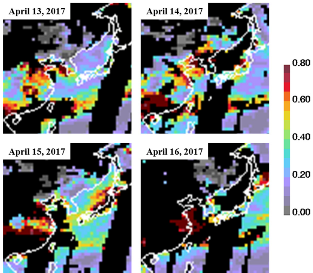
Fig. S1. Aerosol optical depth (AOD) data during intensive periods.
