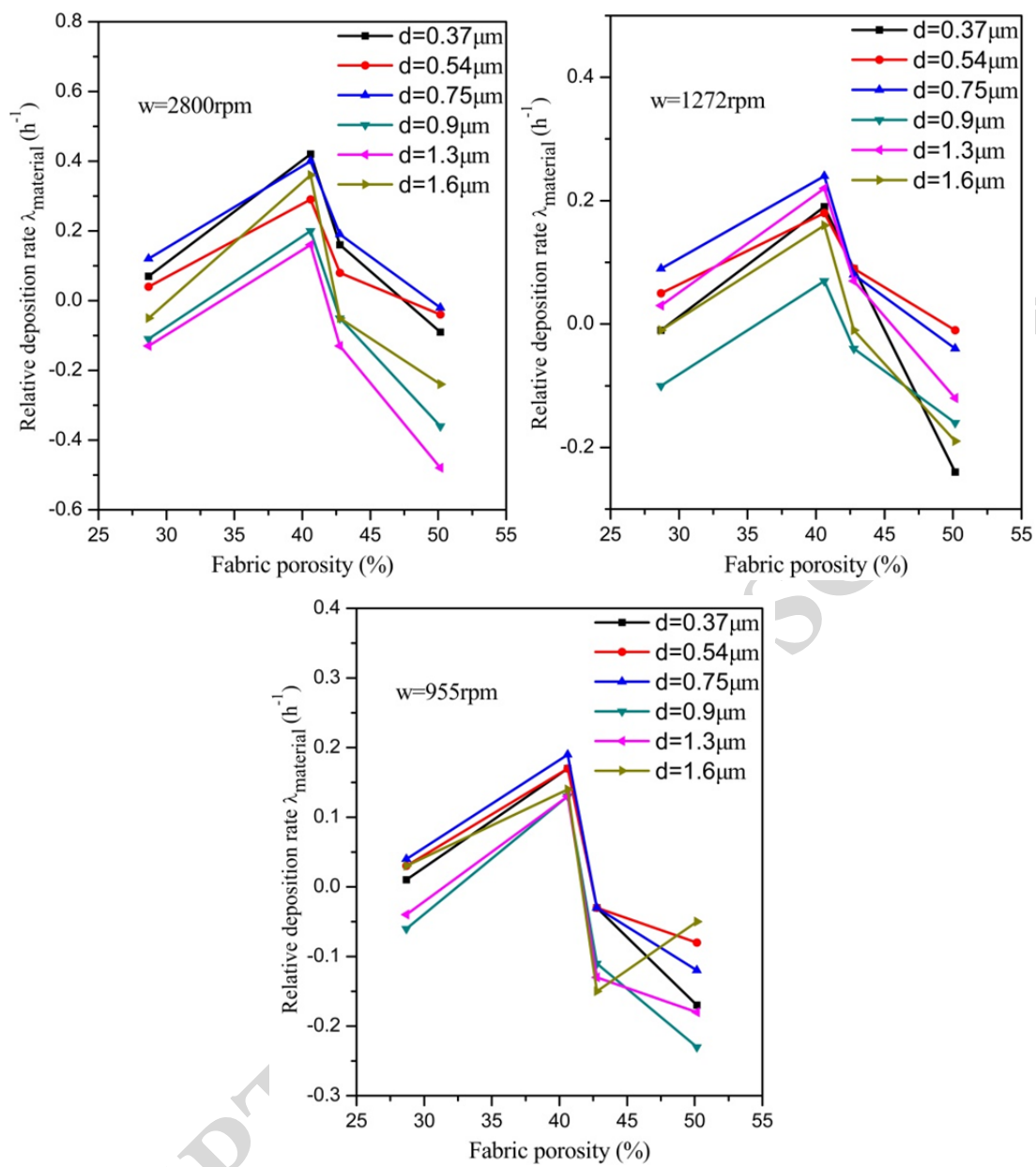
Fig.6. Relative deposition rate \lambda_{\text{material}} versus fabric porosity for samples A to D.
