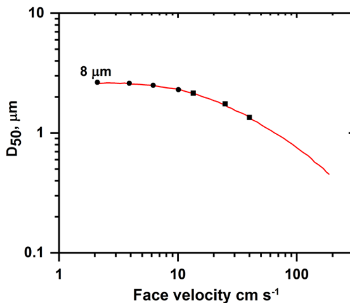
Fig. s1: Variation of the 50% cut point with face velocity for Nuclepore filter, nominal pore size 8.0 μm (data extracted from John et al., 1983).
