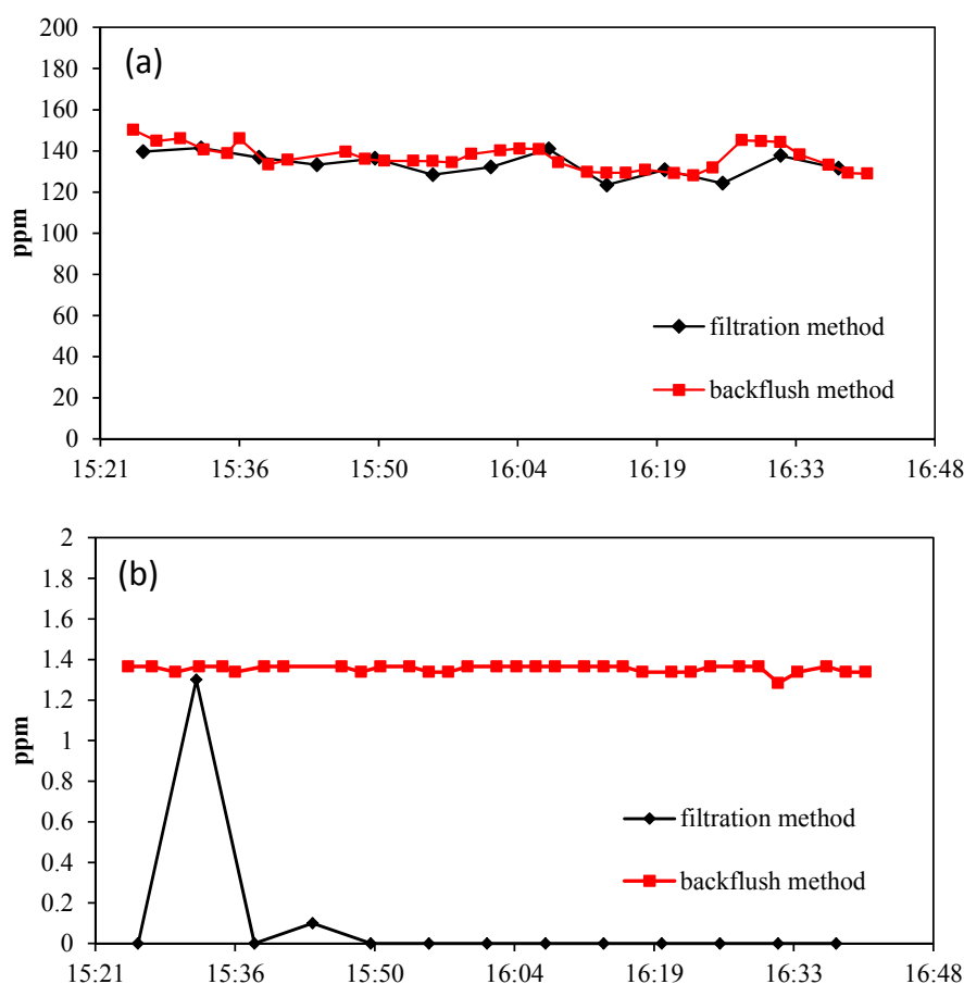
Fig. 6. Continuous monitoring before RTO in a semiconductor fabrication factory. (a) THC measurements; (b) methane measurements. The filtration method was switched between six sampling points of the stack, whereas our back-flush method was only switched between two sampling points, i.e., before and after the RTO unit, resulting in more data points than the filtration method.
