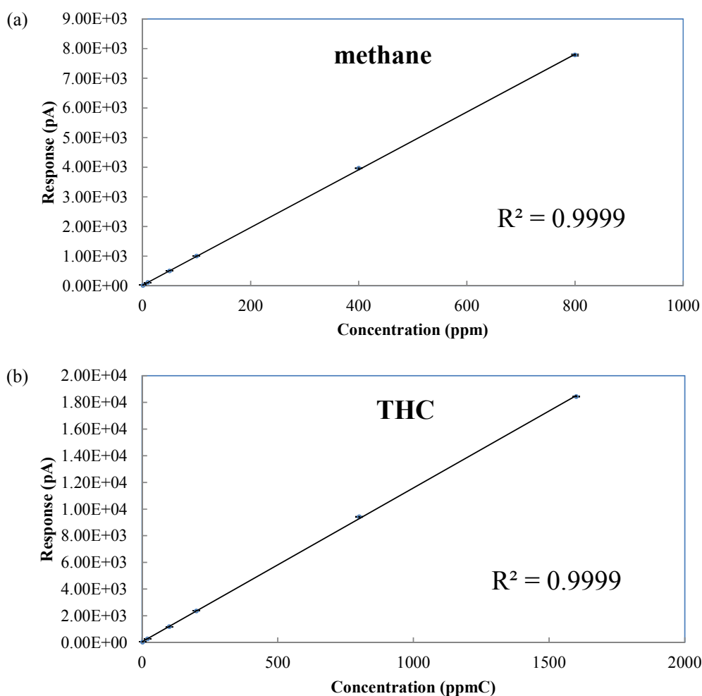
Fig. 5. Calibration curve constructed from 1, 5, 50, 100, 400, 800 ppm for methane (a); and 2, 10, 100, 200, 800 and 1600 ppmC for THC (b). Error bars on the curves are based on five repeated analyses ( N = 5 ) of each standard gas.
