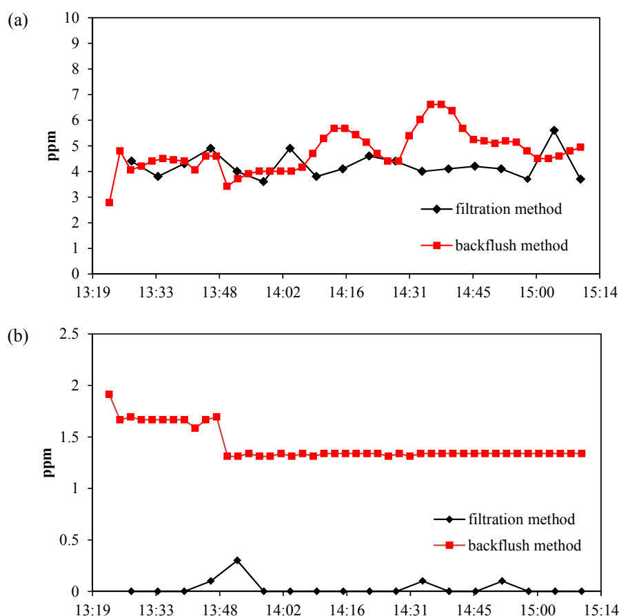
Fig. 7. Continuous monitoring after RTO in a semiconductor fabrication factory. (a) THC measurements; (b) methane measurements.
