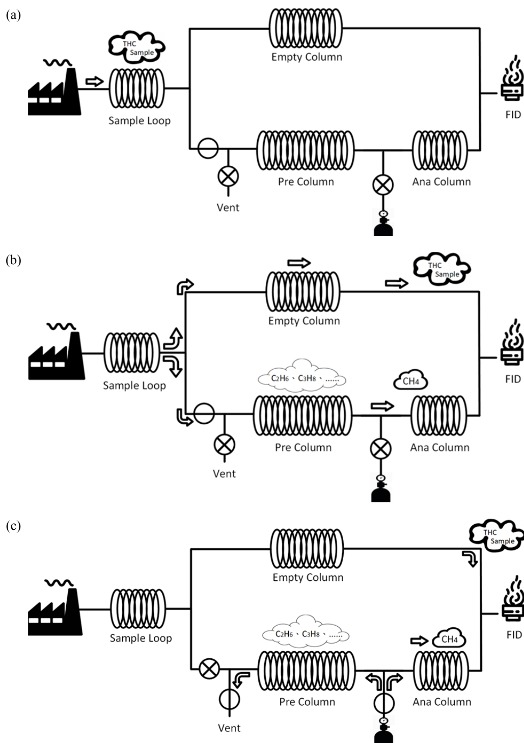
Fig. 2. Schematics of the dual-column GC method during (a) the sample filling stage, (b) the separation stage. Methane is separated and sent to the analytical column while NMHCs are left in the pre-column, and (c) the backflush stage. NMHCs are reversely flushed out of the pre-column while methane is eluting from the analytical column.
