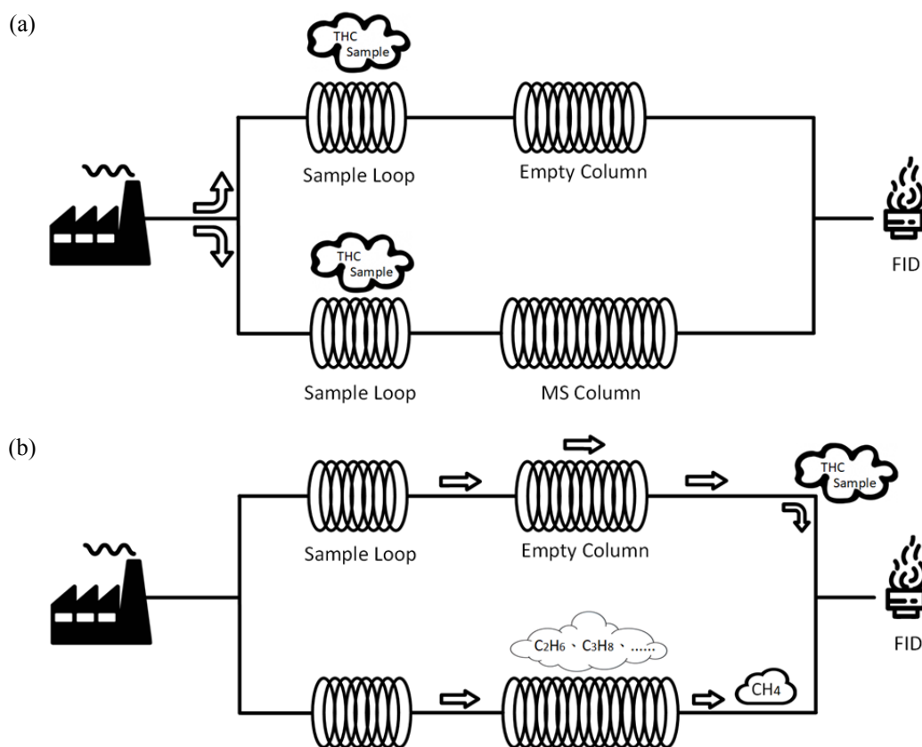
Fig. 1. Schematics of the filtration method during the sample injection stage (a) and the analysis stage. Methane is eluted out of the MS column while other NMHCs are trapped in the MS column (b). MS Column stands for the molecular sieve column and the empty column is an empty s.s. tube.
