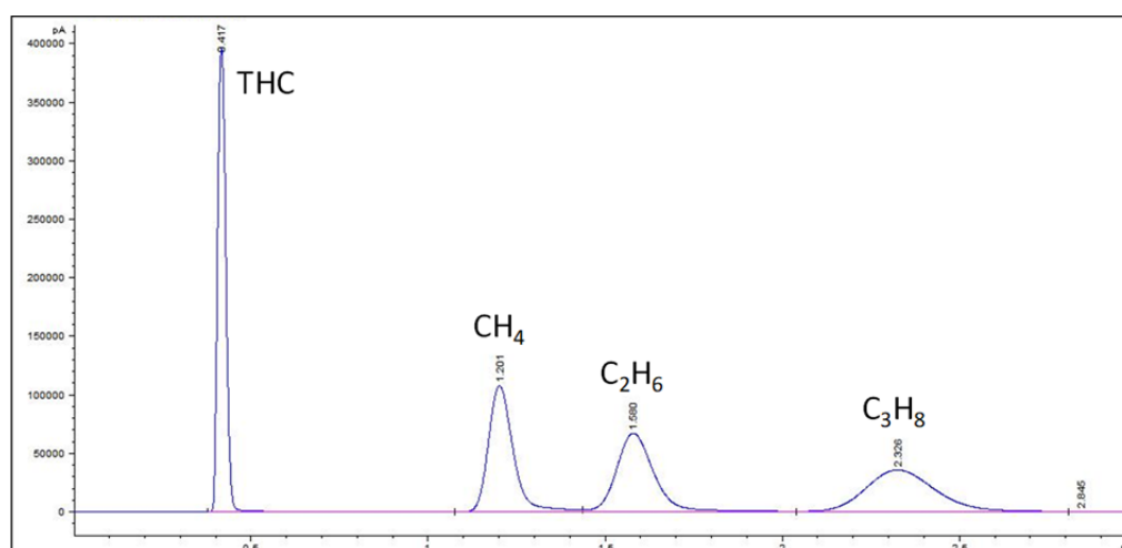
Fig. 3. GC trace of the standard mixture containing methane, ethane and propane. A complete separation of methane from ethane and even propane is clearly shown.
