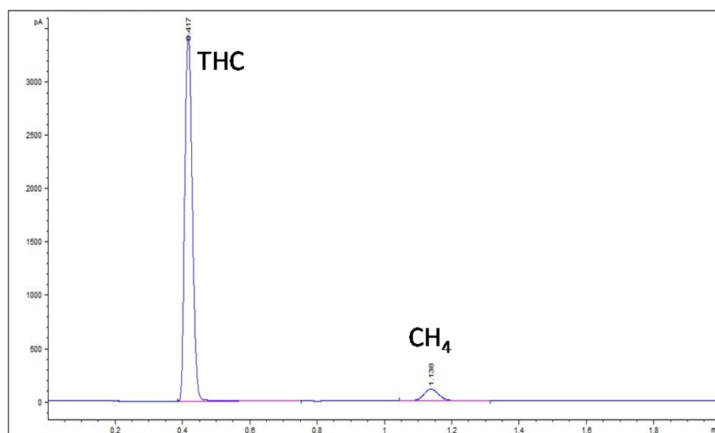
Fig. 4. Back-flush at 0.7 min to only allow methane to come out of the analytical column, while ethane and propane are reversely pushed out of the pre-column to vent. The first tall peak is total hydrocarbons and the second peak is methane.
