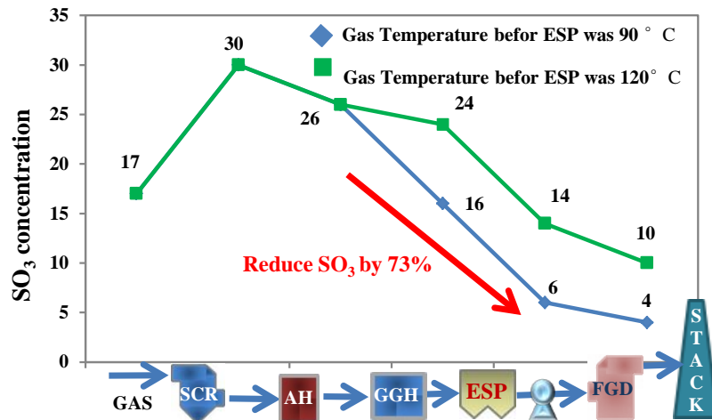
Fig. 6. SO 3 removal performance vs. gas temperature.
