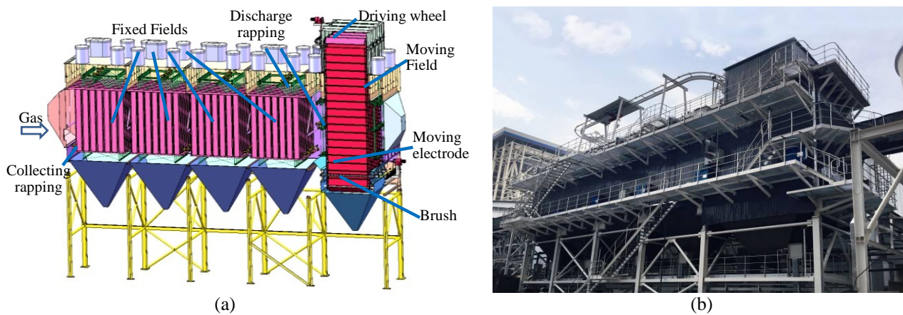
Fig. 2. Sketch of LLT-ESP pilot-plan (a) Schematic diagram and (b) Reality images.
