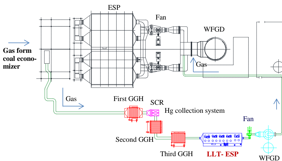
Fig. 1. System diagram of pilot-scale platform.
