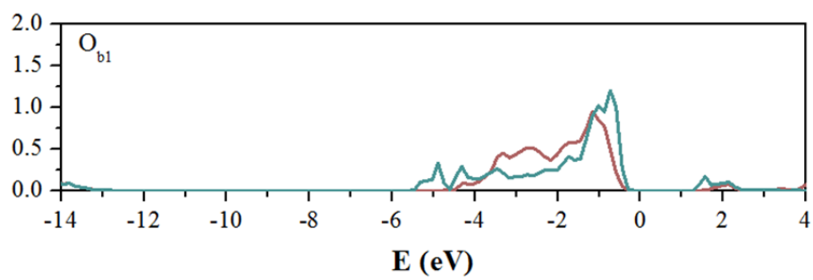
Fig. S2. PDOS for O_{b1} of the Mn-doped CeO_2 (111) surface
