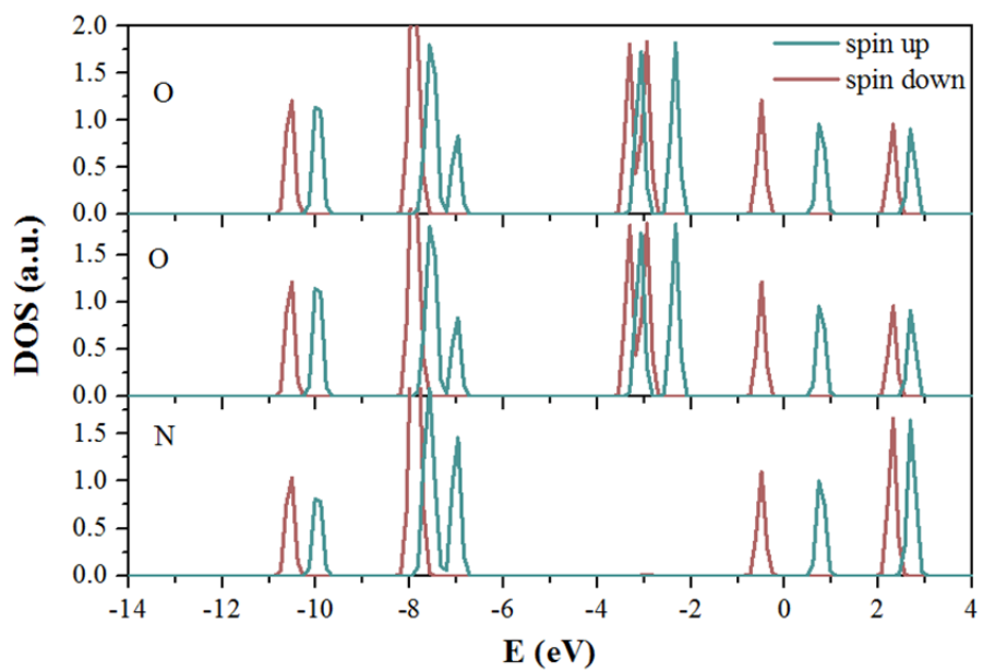
Fig. S1. PDOS for a free NO 2 molecule.
