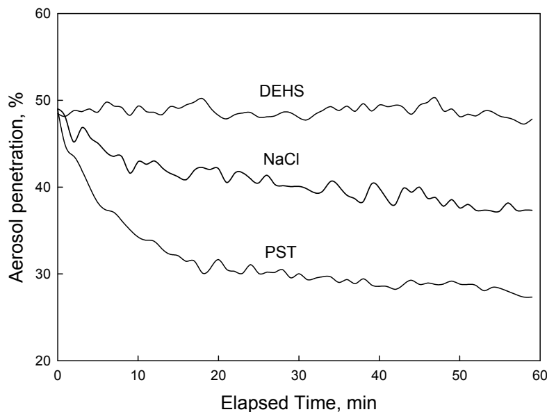
Fig. 4. Penetration of 2.5 \mu\text{m} DEHS, NaCl and PST particles as functions of loading time.
