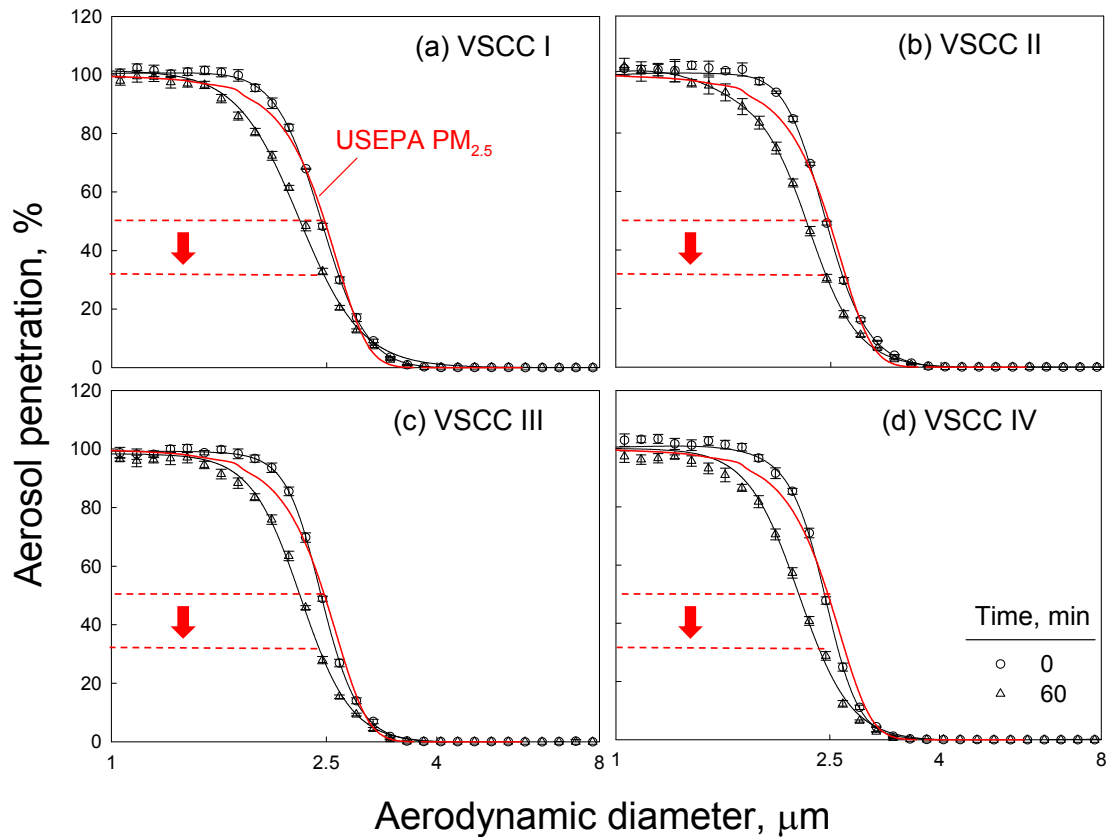
Fig. 7. Separation efficiency curves (initial and after one hour loading) for different-sized cyclones.
