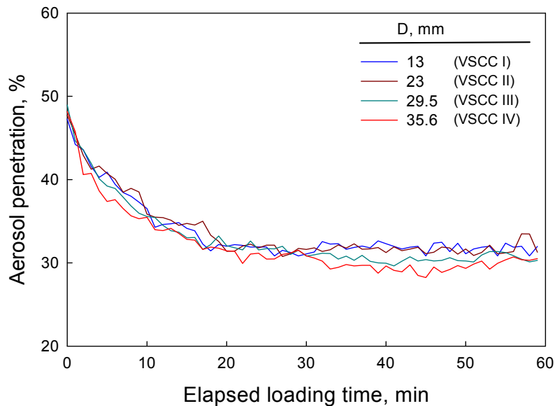
Fig. 8. Penetration of 2.5 \mu\text{m} PST particles through four different-sized cyclones as a function of loading time.
