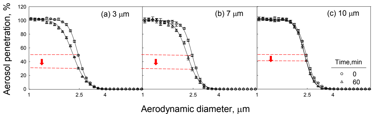
Fig. 5. Separation efficiency curves (initial and after one hour loading) for different sizes of PST particles through a VSCC III sampler.
