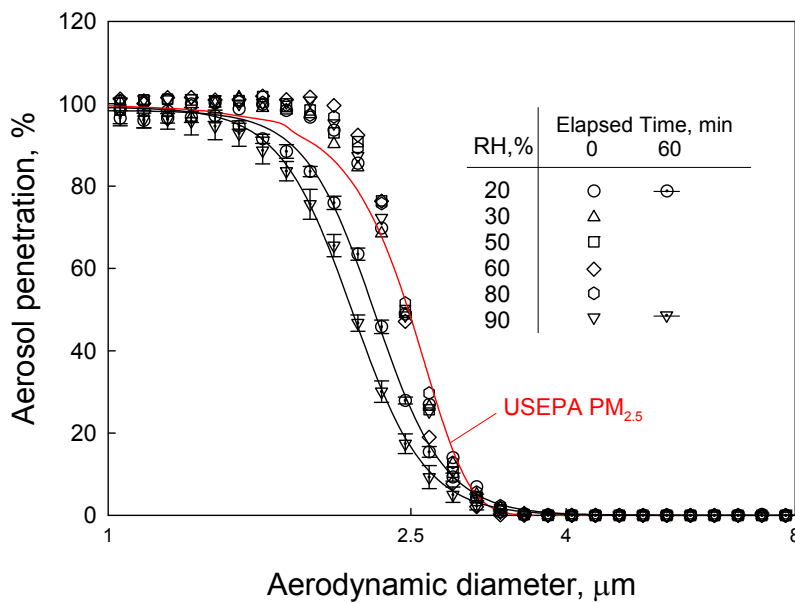
Fig. 9. Separation efficiency curves (initial and after one hour loading) under different relative humidities.
