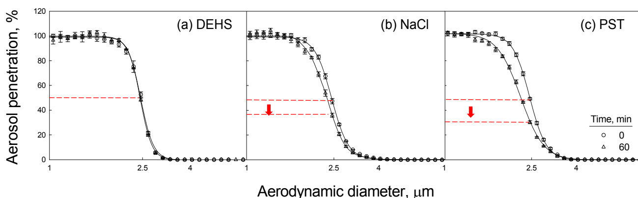
Fig. 3. Separation efficiency curves (initial and after one hour loading) for different kinds of loading particles.
