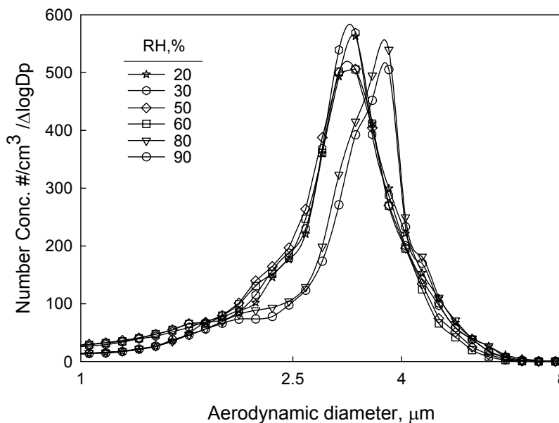
Fig. 10. Size distributions of PST particles under different air humidities.
