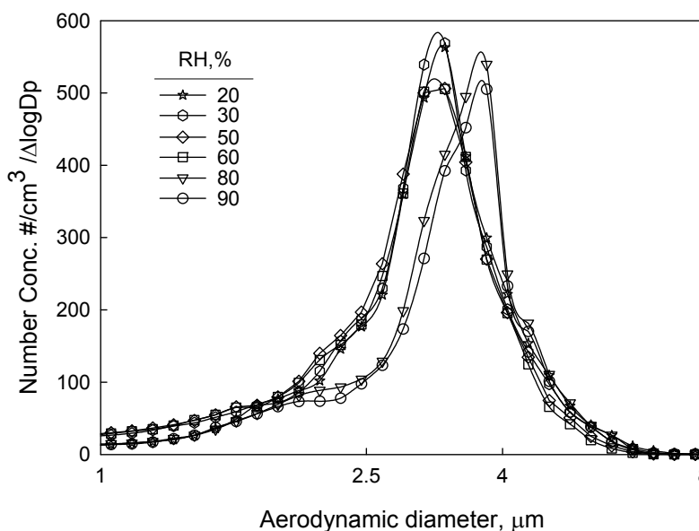
Fig. 10. Size distributions of PST particles under different air humidities.
