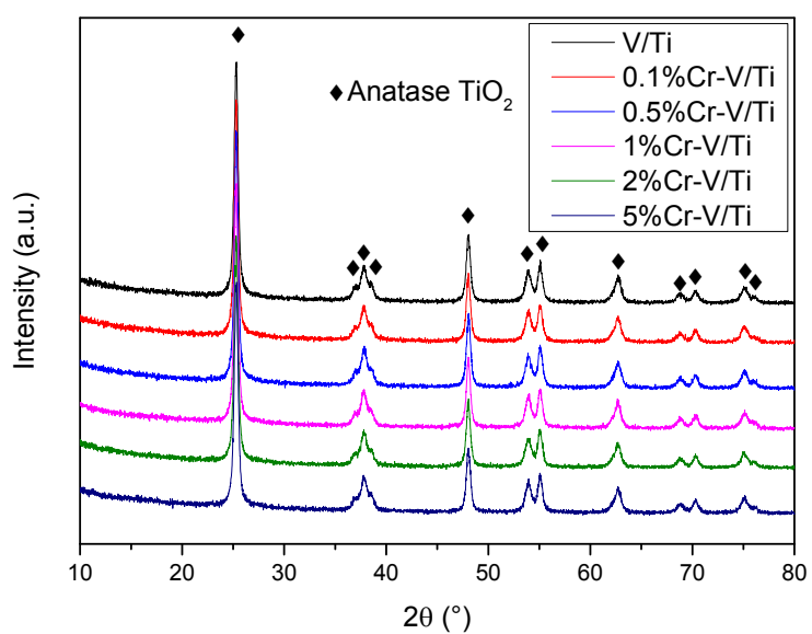
Fig. 1. XRD patterns of Cr-V/Ti catalysts.
