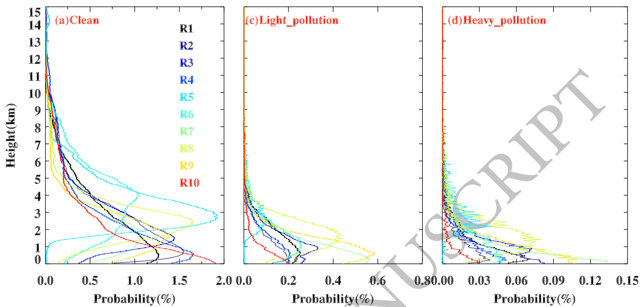
Figure 3 Annual average vertical profiles of probability of occurrence for clean, light-polluted, and heavy-polluted conditions in the 10 regions.
