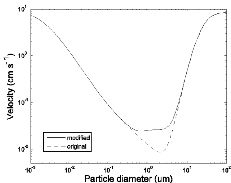
Fig. 1. Size-resolved V_d from the modified and the original models.
