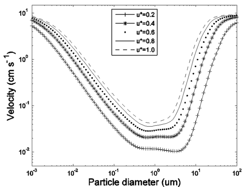
Fig. 2. Modeled size-resolved V_d under different u_* conditions.
