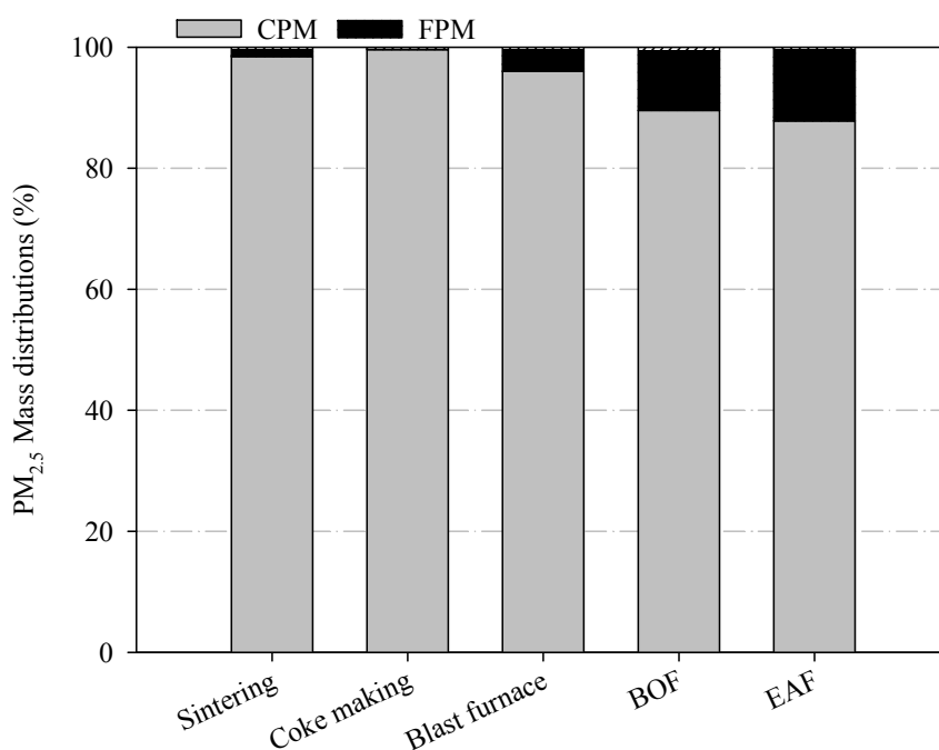
Fig. 2. Partitions of filterable and condensable PM 2.5 for the plants.
