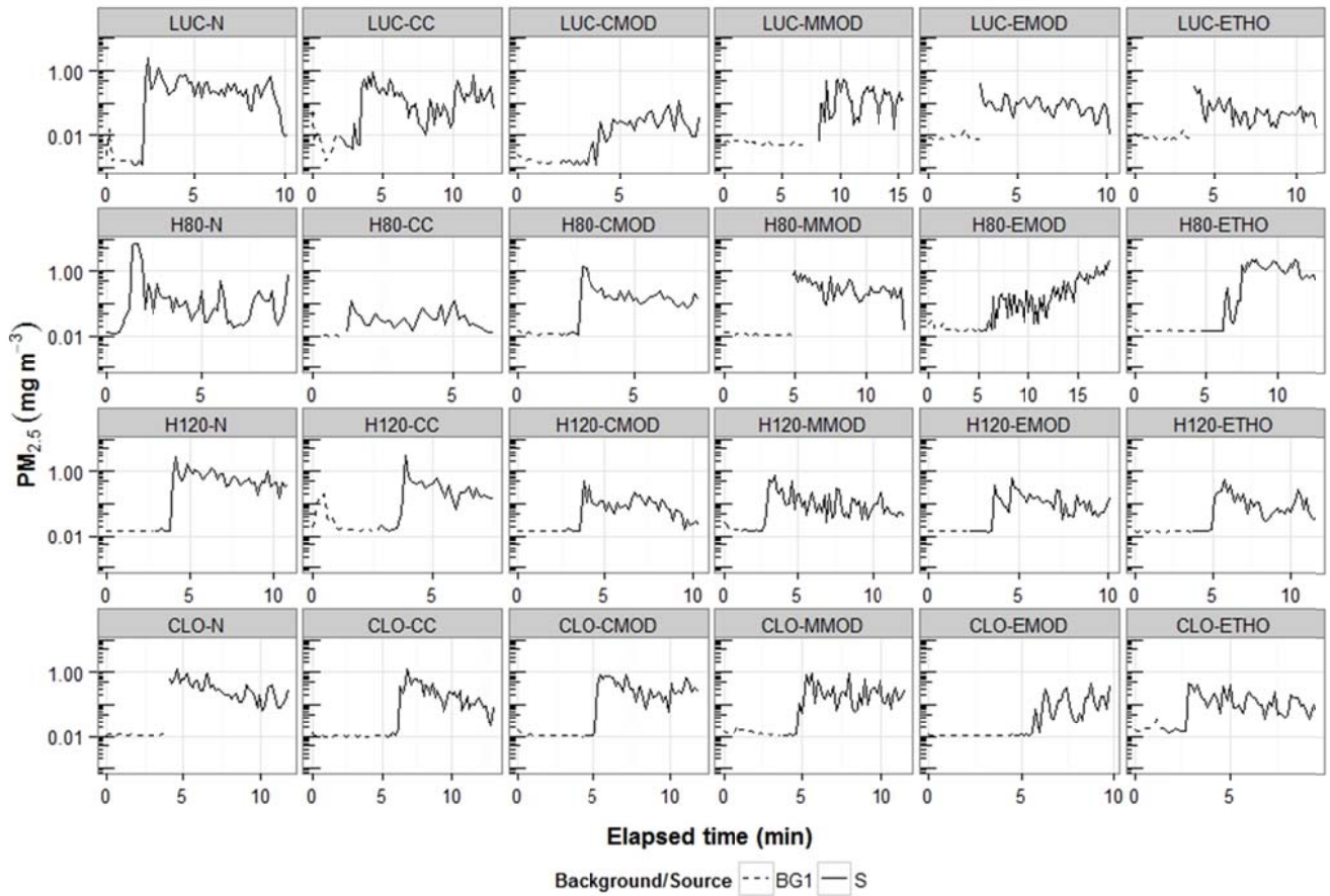
Fig. 10. 10-second averaged time-series of source PM_{2.5} for all primary particle size/surface treatment combinations.
