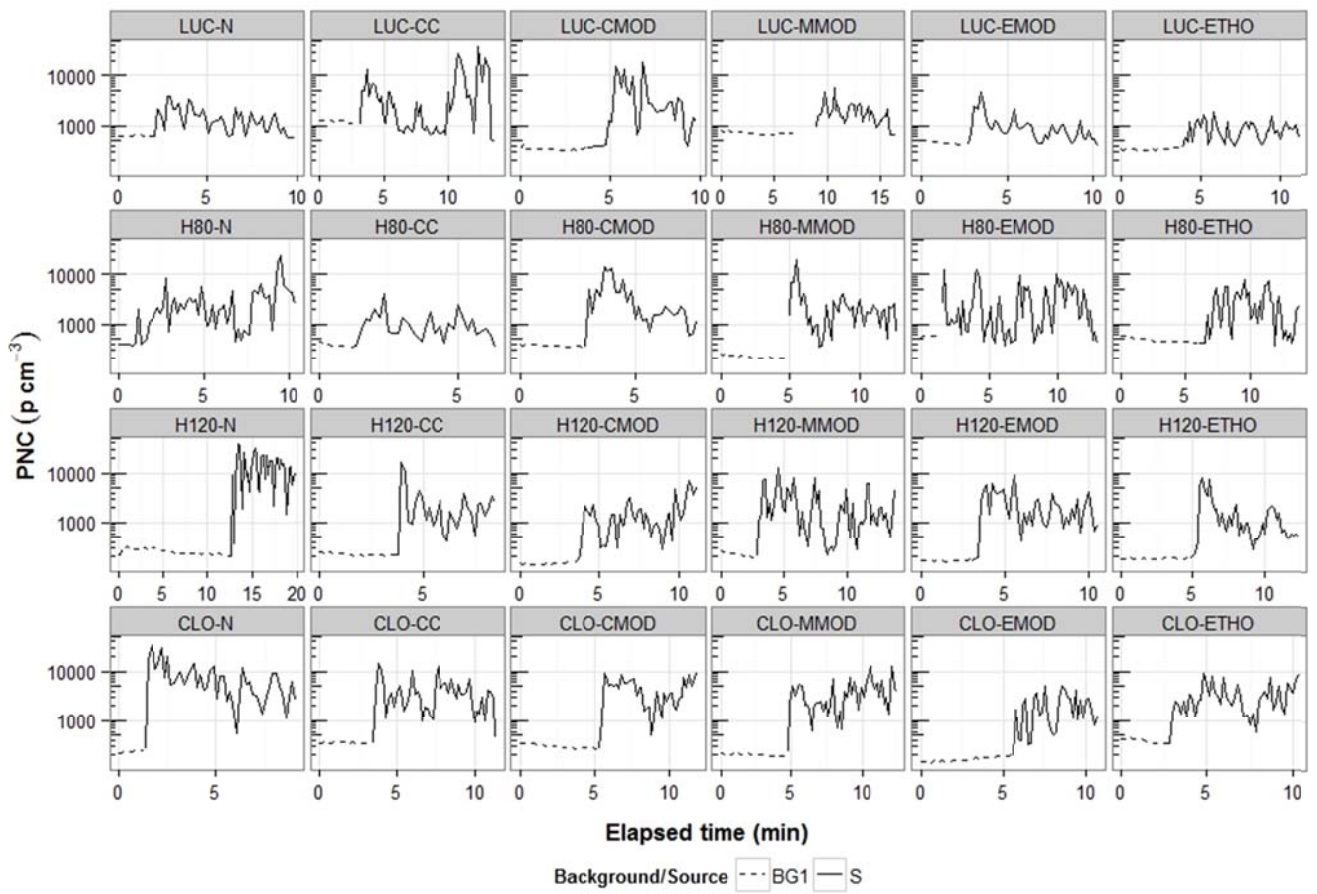
Fig. 11. 10-second averaged time-series of source PNC for all primary particle size/surface treatment combinations.
