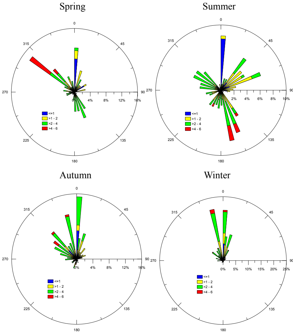
Figure S1. Wind rose during the study period.
