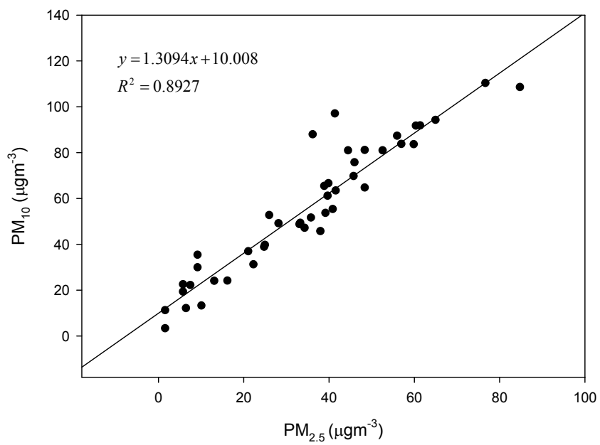
Figure S2. Correlation between PM_{2.5} and PM_{10} in the sampling site.
