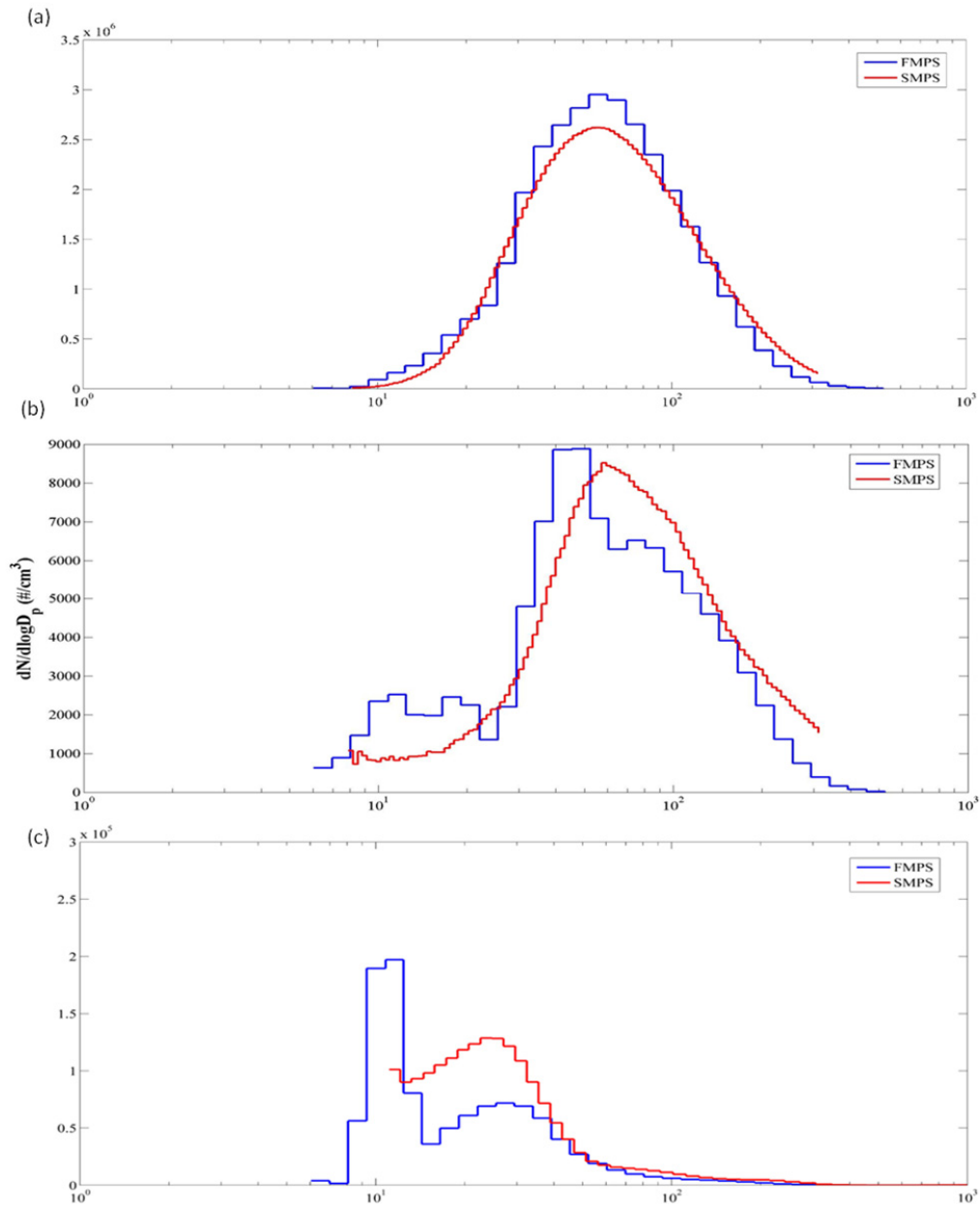
Fig. S1. Results of inter-instrument comparison between FMPS and SMPS on (a) chamber of 0.5 % (\text{NH}_4)_2\text{SO}_4 nanoparticles, (b) suburban indoor and (c) outdoor.
