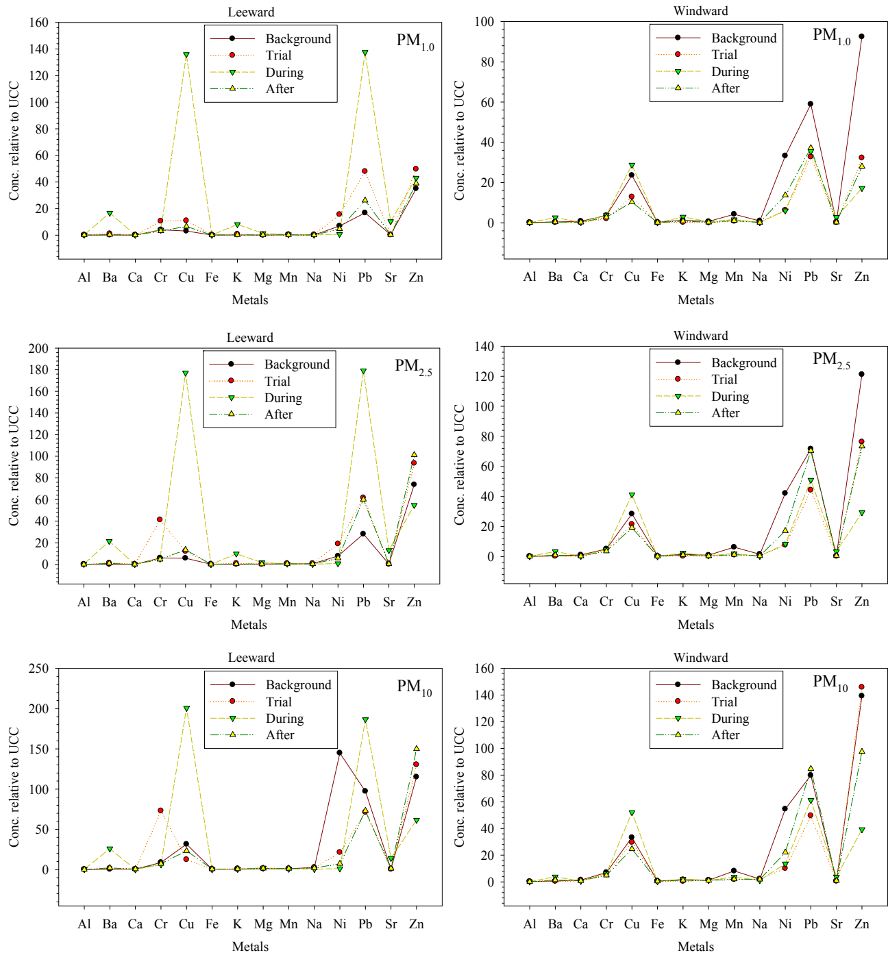
Fig. 2. Metals distribution patterns (normalized to upper continental crust (UCC)) for the sized particles at the leeward and windward sampling sites.
