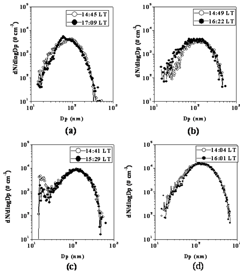
Fig. 17. Size distributions of aerosol particles measured by SMPS, at very low aerosol mass concentration was measured during the day. Graph represent (a) 2 nd August, monsoon, (b) 21 st October, post-monsoon (c) 14 th January, a typical hazy day (d) 9 th December a typical foggy day.
