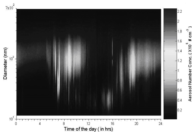
Fig. 11. Contour graph for the typical foggy day in winter season, showing the diurnal variation of the number concentration and size distribution on 25.12.2006.
