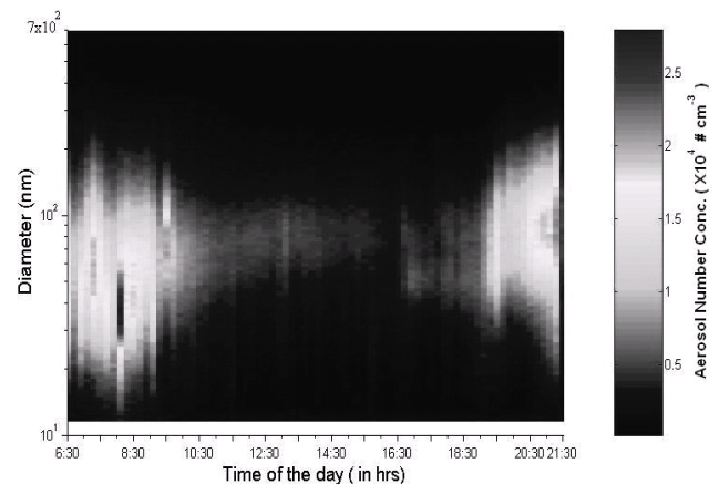
Fig. 3. Contour graph for the typical monsoon day, showing the diurnal variation of the number concentration and size distribution on 2.08.2006.
