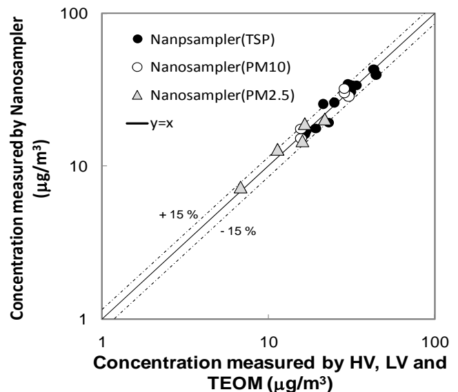
Fig. 6. Comparison of particle concentrations in different size ranges obtained by Nanosampler with those by other samplers.
