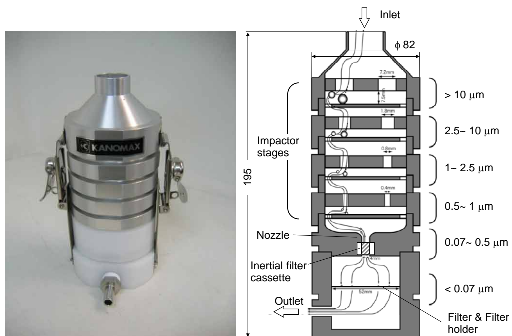
Fig. 1. Schematic drawing and picture of Nanosampler.
