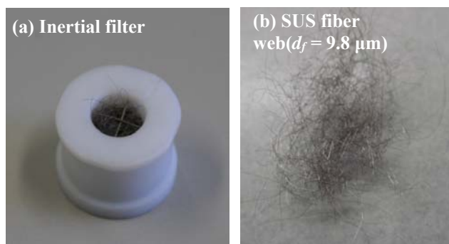
Fig. 2. Inertial filter cartridge along with SUS fiber web. (a) Inertial filter cartridge along with SUS fiber web. (b) SUS fiber web ( d_f = 9.8 \mu\text{m} ).
